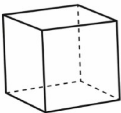
cube
