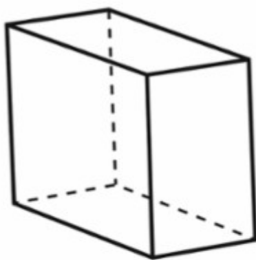
rectangular prism
