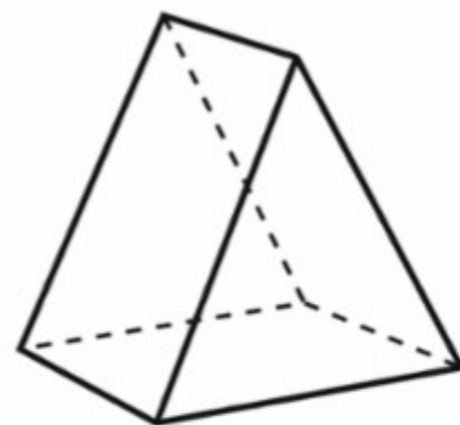
triangular prism
